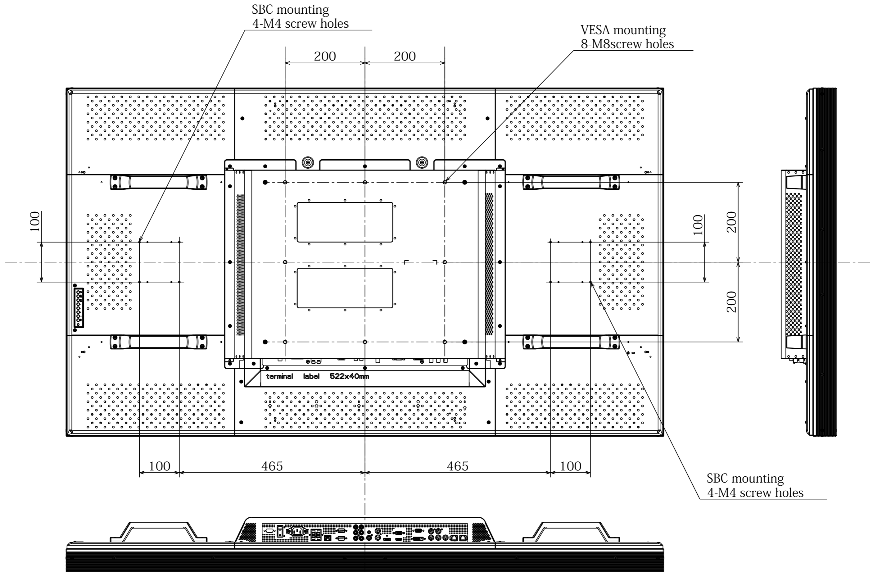
MDT652S OUTLINE 2011/4/15 (2/2)
