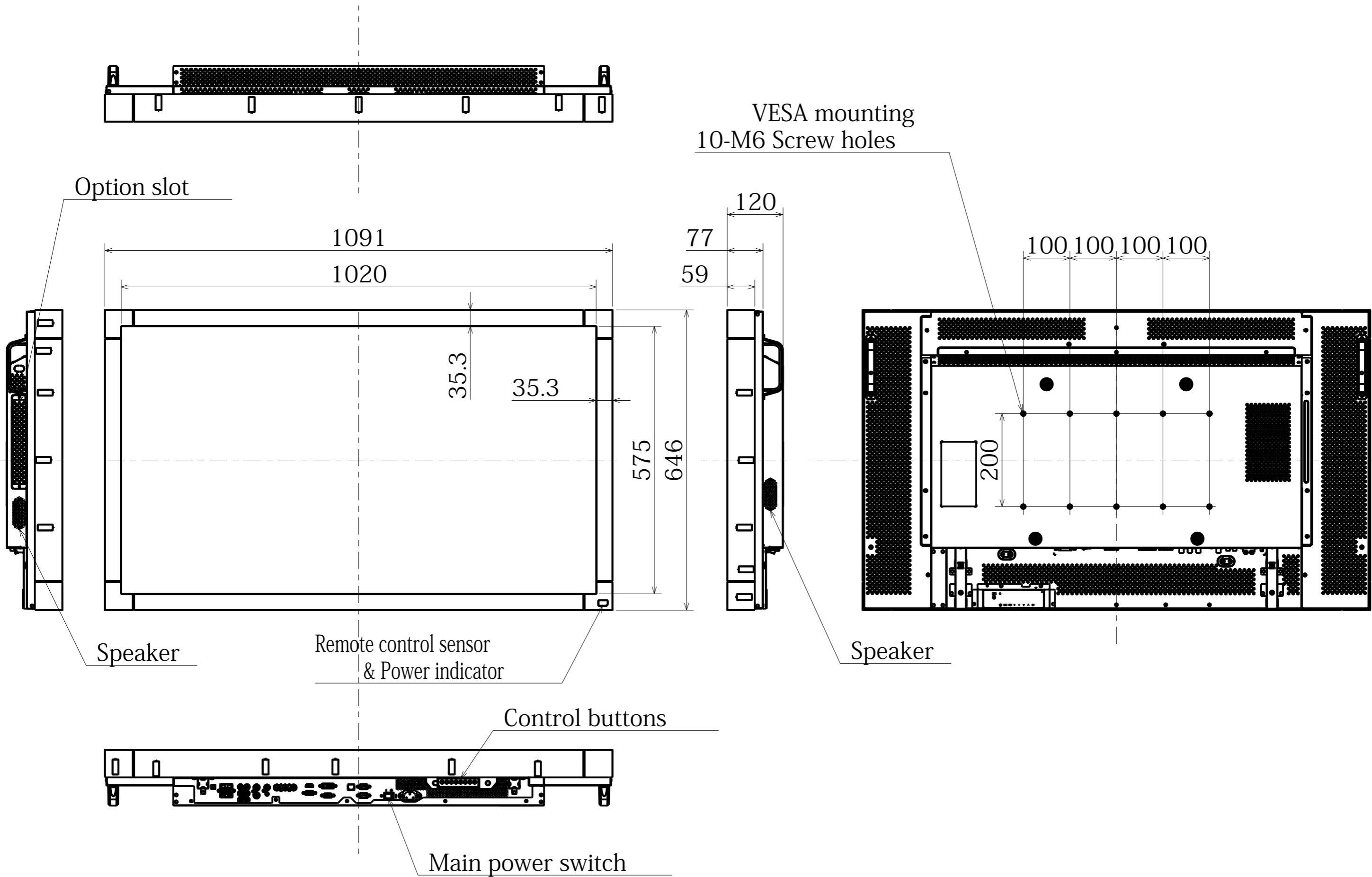
LDT462V OUTLINE 2012/1/6
